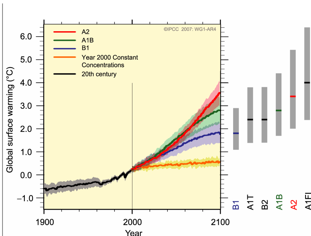
Figure IV.18. Multi-model averages and assessed ranges for surface warming. Solid lines are multi-model global averages of surface warming (relative to 1980 to 1999) for the scenarios A2, A1B, and B1, shown as continuations of the 20th-century simulations. Shading denotes the \pm 1 standard deviation range of individual model annual averages. The orange line is for the experiment where concentrations were held constant at year 2000 values. The grey bars at right indicate the best estimate (solid line within each bar) and the likely range assessed for the six SRES marker scenarios. The assessment of the best estimate and likely ranges in the grey bars includes results from the atmosphere–ocean general circulation models shown in the left part of the figure, as well as results from a hierarchy of independent models and observational constraints. Source: IPCC (2007d).
